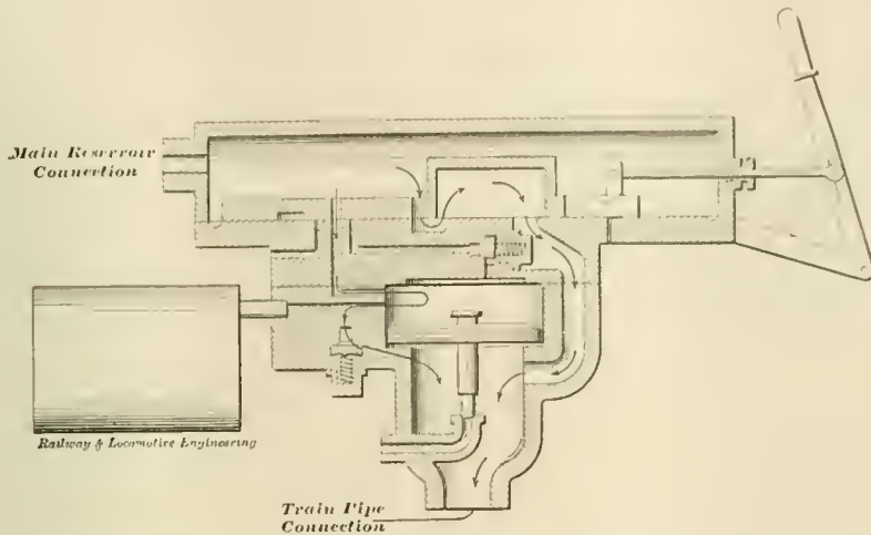
NEWLY PATENTED BRAKE VALVE—FULL RELEASE POSITION.
